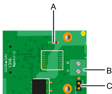
Figure 23 : carte de communication RS485
