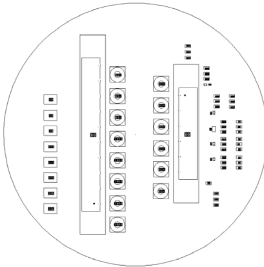
Figure 2-12 Terminals
